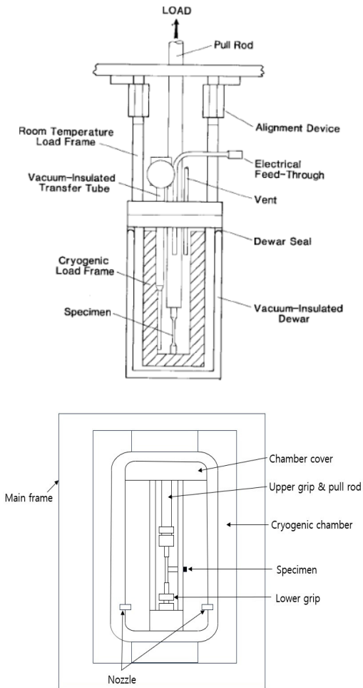
Fig. 1. Schematic illustrations of typical cryostat for tension testing (a), and used in study (b)
