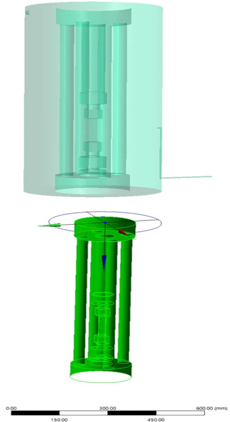
Fig. 2. Geometry model of cryogenic chamber
