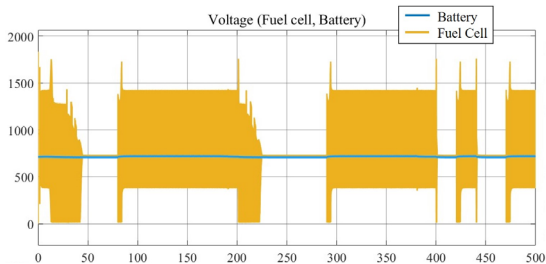
Fig. 12. Output voltage of fuel cell and battery at gross combination weight vehicle
