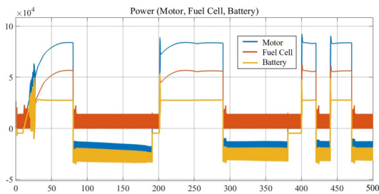
Fig. 4. Output power of motor, fuel cell, and battery at curb weight vehicle
