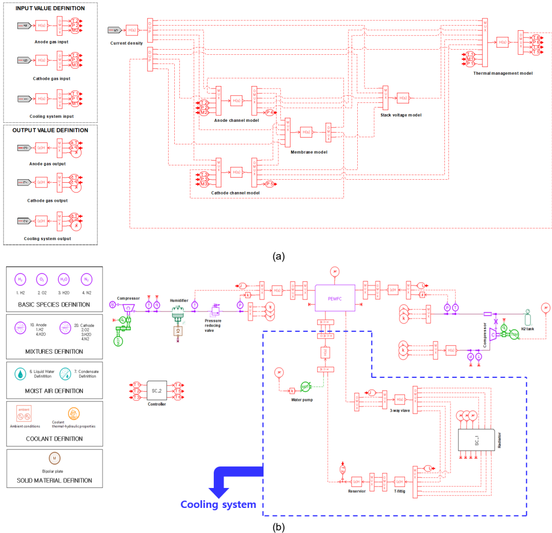
Fig. 2. Modeling of PEMFC system model using AMESim. (a) Stack model using AMESim, (b) fuel cell system model with cooling system using AMESim
