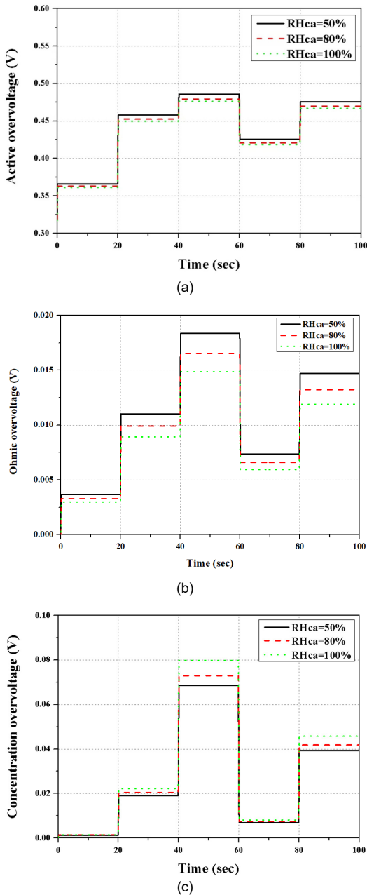
Fig. 10. Analysis of stack voltage loss by humidity. (a) Active overvoltage, (b) ohmic overvoltage, (c) concentration overvoltage
