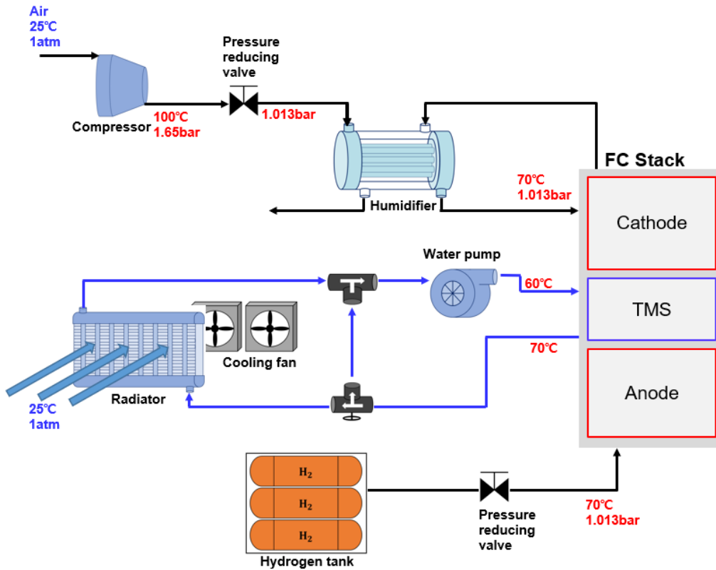
Fig. 1. Schematic diagram of fuel cell system
