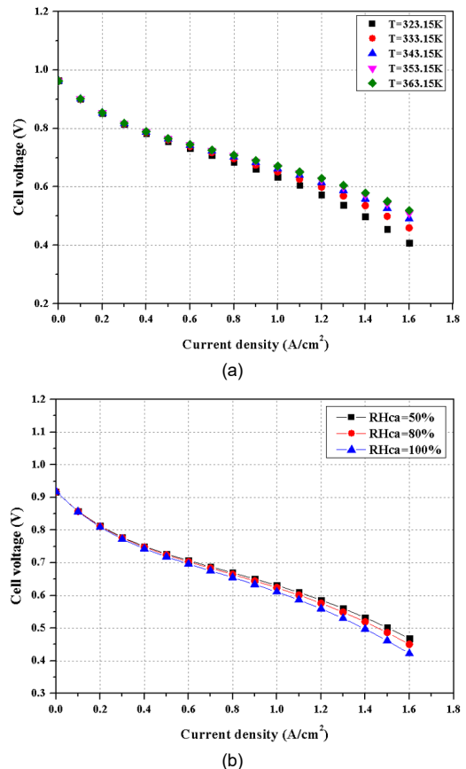
Fig. 11. Voltage performance of the stack according to operating conditions. (a) Voltage performance with temperature, (b) voltage performance with humidity
