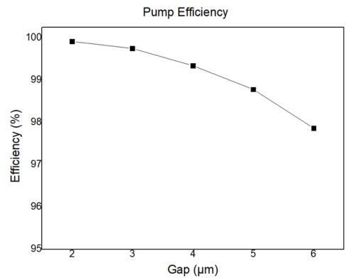
Fig. 8. Efficiency graph
