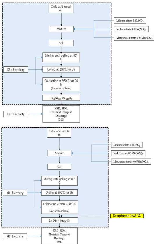
Fig. 4. Process flow diagram for Li_{1.6}Ni_{0.35}Mn_{0.65}O_2 and Li_{1.6}Ni_{0.35}Mn_{0.65}O_2 & graphene 2wt%
