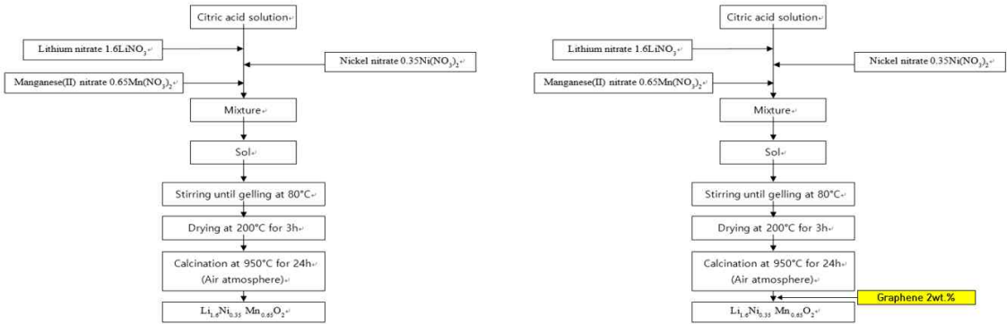
Fig. 1. Flow charts of experimental procedure of \text{Li}_{1.6}\text{Ni}_{0.35}\text{Mn}_{0.65}\text{O}_2 and \text{Li}_{1.6}\text{Ni}_{0.35}\text{Mn}_{0.65}\text{O}_2 & graphene 2wt%
