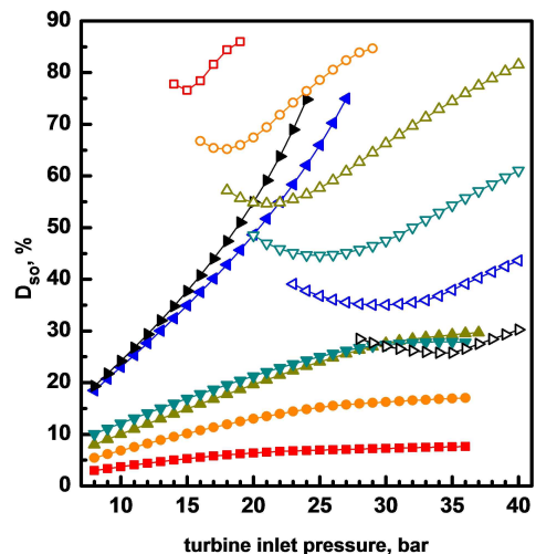
Fig. 2. Effects of turbine inlet pressure on the exergy loss ratio of source exhaust, D_{s0} .
