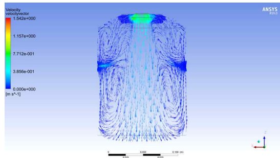
Fig. 4. Velocity profiles in the mixing compartment
