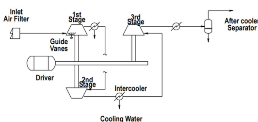
Fig. 2. Schematic diagram for MAC with inter-coolers using cooling water
