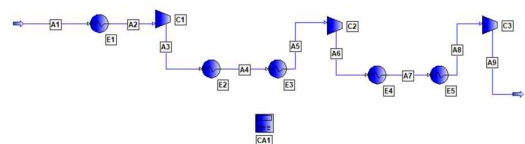
Fig. 6. PRO/II flow sheet drawing for MAC with pre-cooler and inter-coolers using both cooling water and refrigerant
